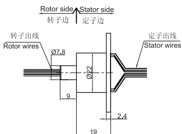
MC190-FL02图纸
