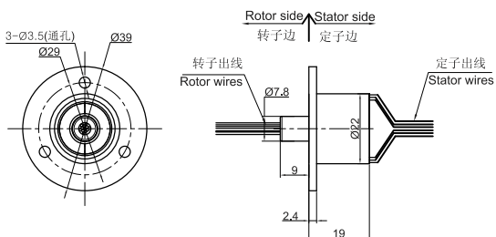
MC190-FL04图纸
