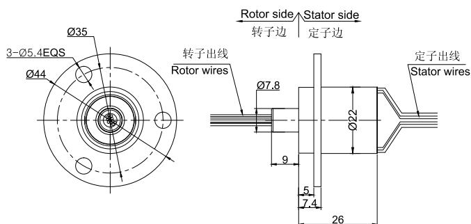
MC260图纸
