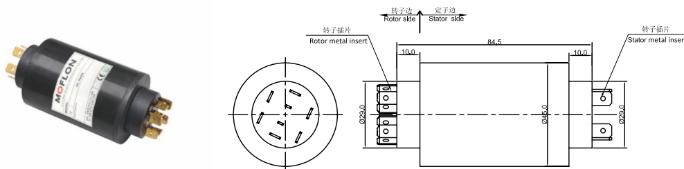
MW4045-P0630-P0208 尺寸图
