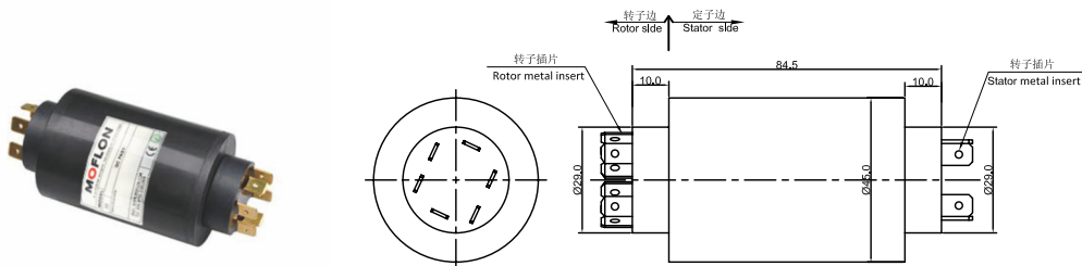
MW4045-P0430-P0208 尺寸图
