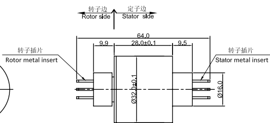
MW4032-P0230-P0208 尺寸图
