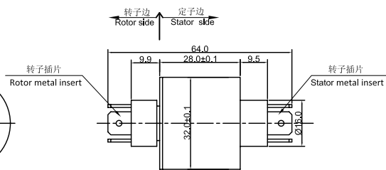
MW4032-P0230-P0208 尺寸图
